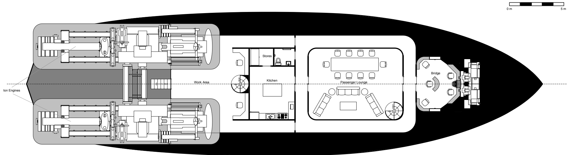
DECK PLANS - LEVEL 1 (Bridge and Lounge)
