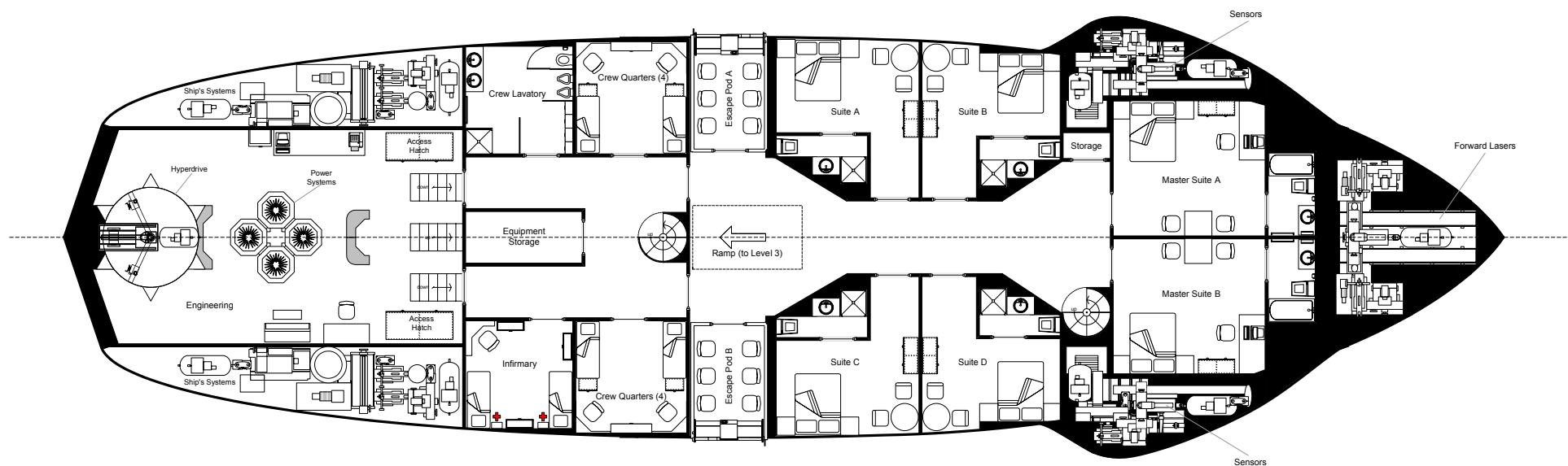
DECK PLANS - LEVEL 2 (Living Quarters and Engineering)
