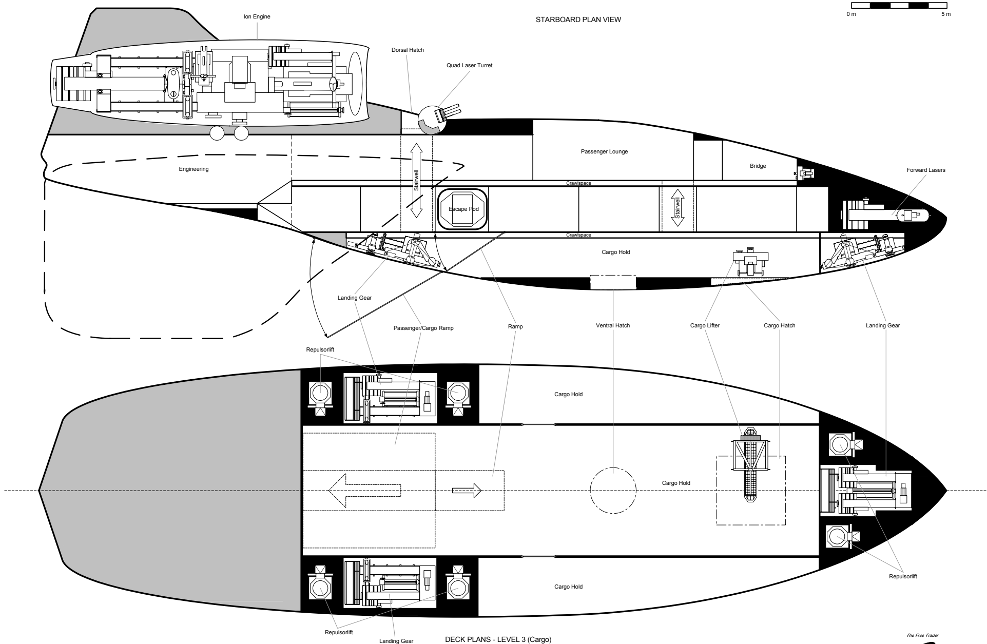
DECK PLANS - LEVEL 3 (Cargo)
